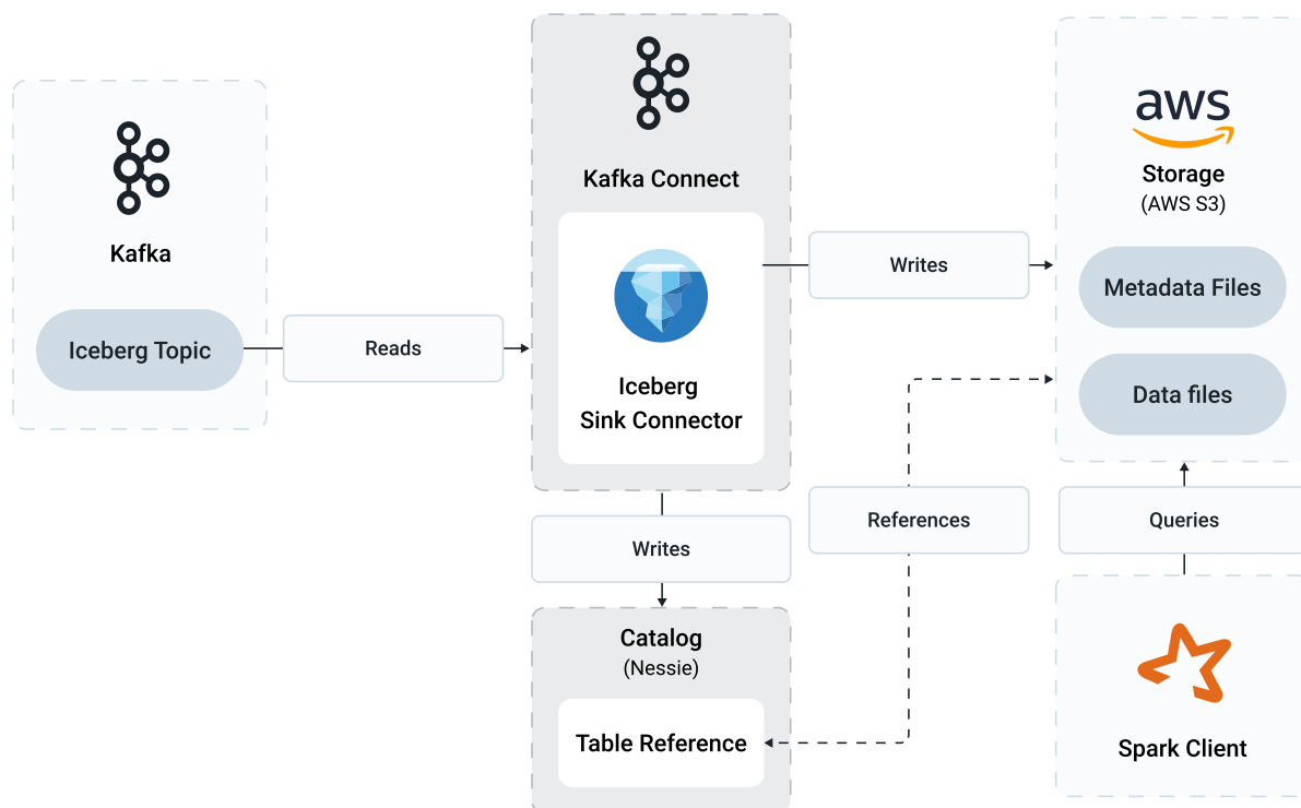
Figure 1: Apache Iceberg Sink Connector example deployment
